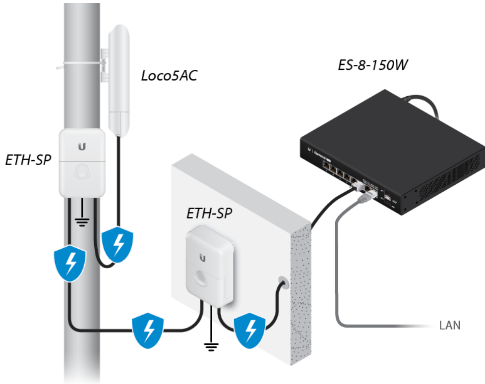
Diagram Showing Use of Ethernet Surge Protectors
